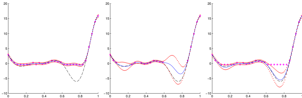
Figure 2: Regression with censored data. Left panel: standard GP model on data with censored samples. Middle panel: standard GP model on data where censored samples were removed. Right panel: Tobit GP model on data with censored samples. The * denotes observations (possibly noisy and/or censored). Dashed line denotes the underlying true function. Solid line denotes the mean model prediction. Dotted line denotes two standard deviations from the mean.
